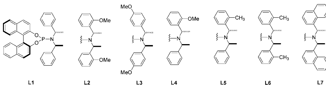
Figure 1. Chiral ligands used in this study.
