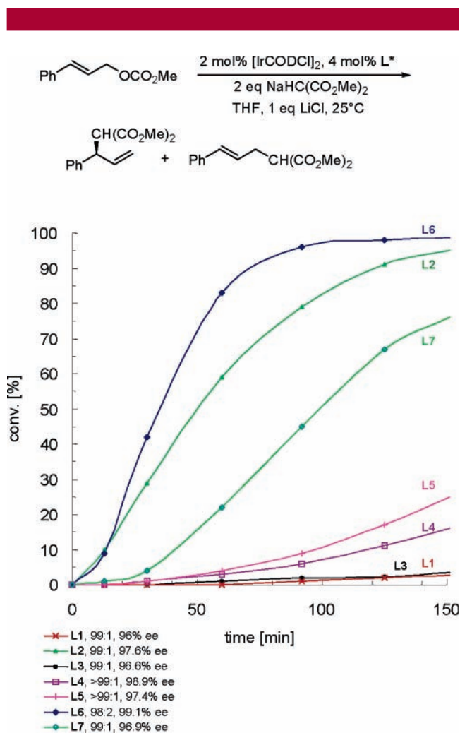
Figure 3. Comparison of the kinetics of the catalysts resulting from the corresponding ligands in the Ir-catalyzed allylic alkylation with sodium dimethylmalonate.
