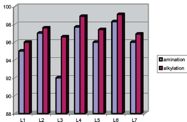
Figure 4. Recapitulative comparison of the ee's (%) resulting from the Ir-catalyzed allylic amination with benzylamine and alkylation with sodium dimethylmalonate with ligands L1 – L7 .
