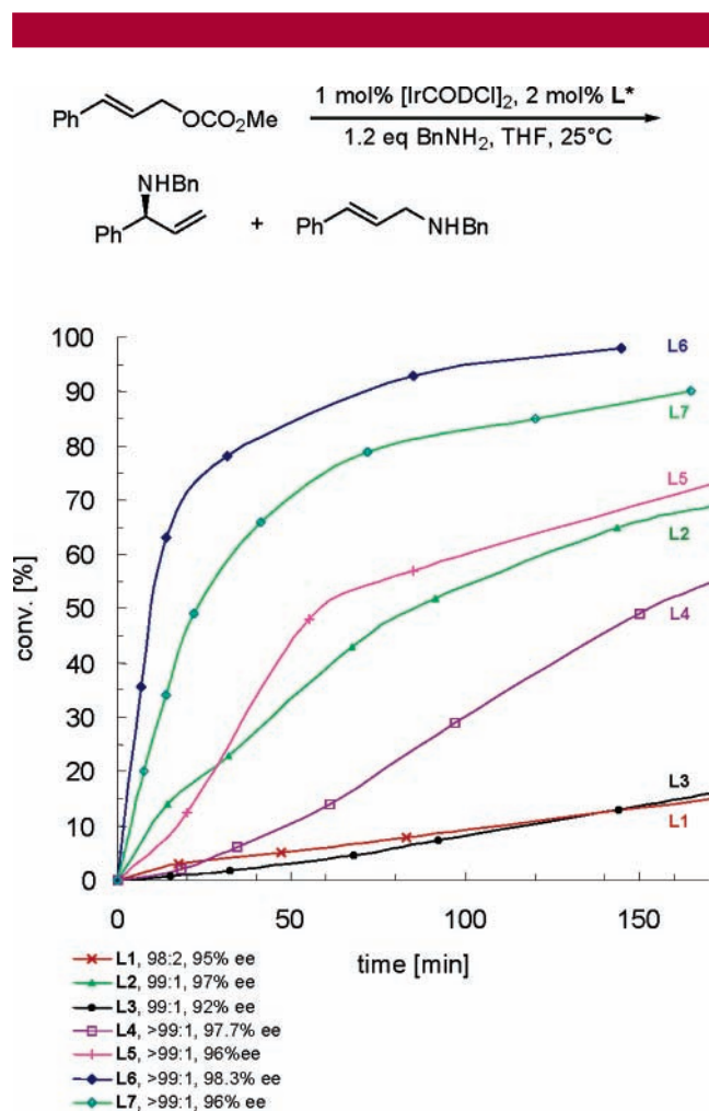
Figure 2. Comparison of the kinetics of the catalysts resulting from the corresponding ligands in the Ir-catalyzed allylic amination with benzylamine.
